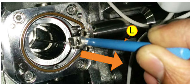
Figure 10-14: Removing the Wave Guide (Generic View)
