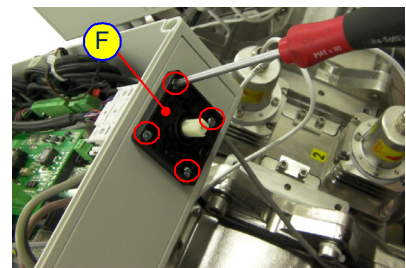
Figure 5-38: Replacing the Power Cable 3
