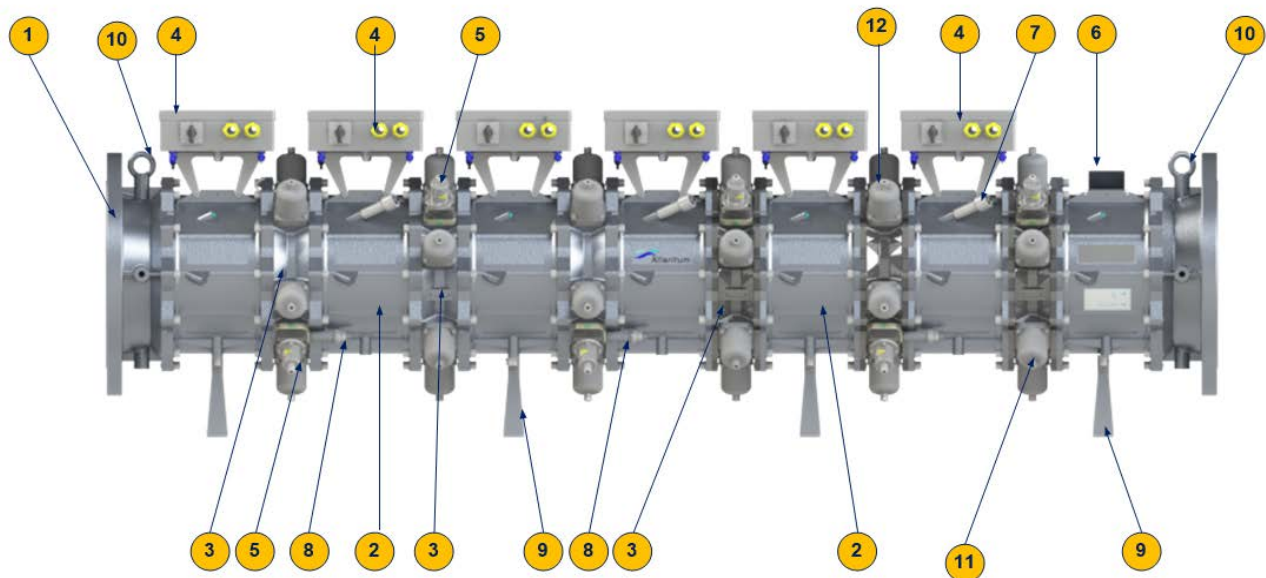
Figure 2-1: RZ300 with Ultrasonic Cleaner
