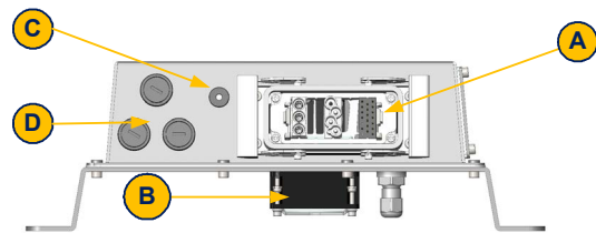
Figure 5-17: Ballast Module C-Waterproof Box (bottom view)
