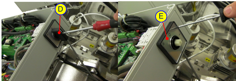
Figure 5-36: Replacing the Power Cable 1
