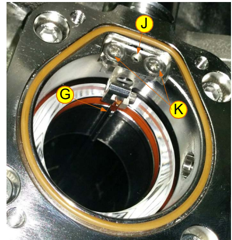
Figure 10-13: Wave Guide Elements (Generic View)
