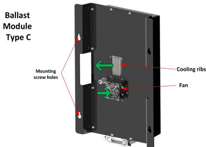
Figure 10-5: Accessing cooling fans
