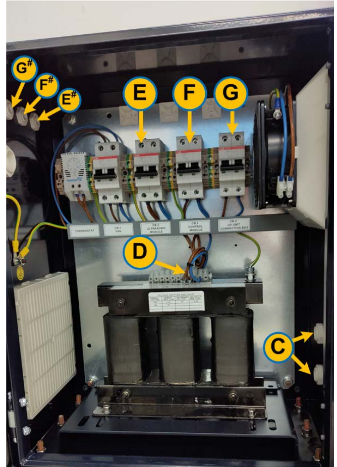
Figure 5-26: Power Module - connections
