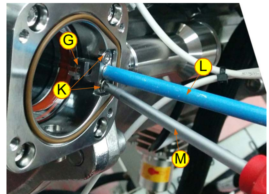
Figure 10-15: Unfastening the Wave Guide (Generic View)
