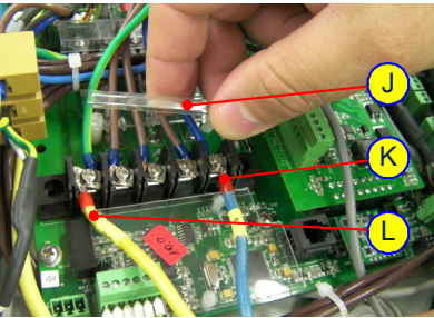
Figure 5-40: Replacing the Power Cable 5
