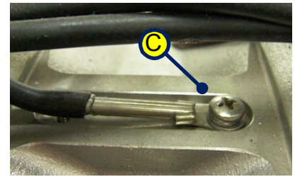
Figure 10-35: Location of the Temperature Sensor on the Atlantium Unit
