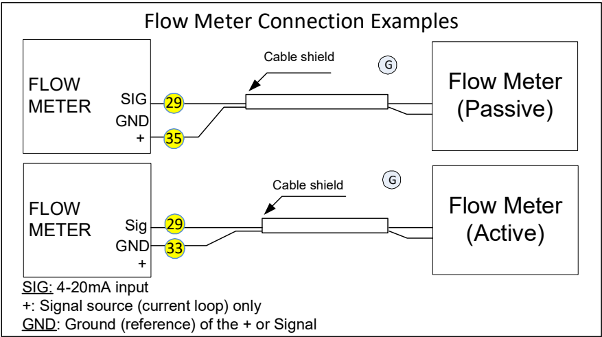
Figure 5-33: Flow Meter Connection Examples
