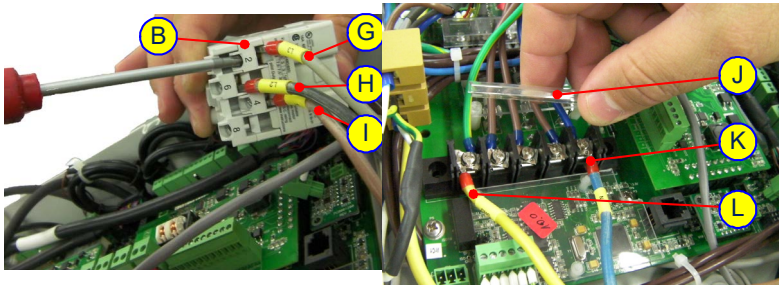
Figure 5-39: Replacing the Power Cable 4
