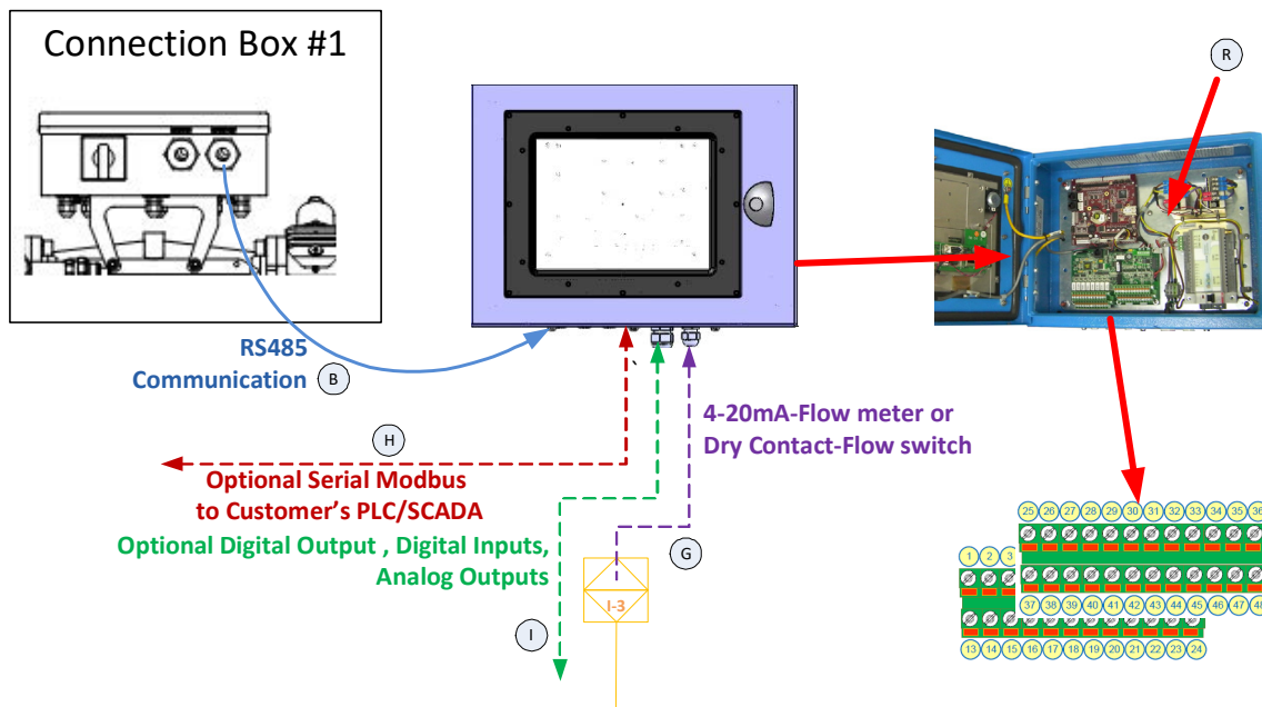
Figure 5-31: Digital and Analog Input and Output Connections-Schematic Diagram
