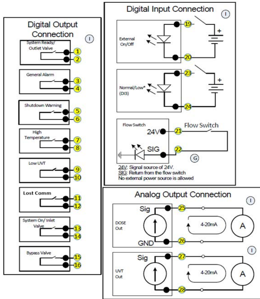
Figure 5-32: Digital and Analog Input and Output Connections
