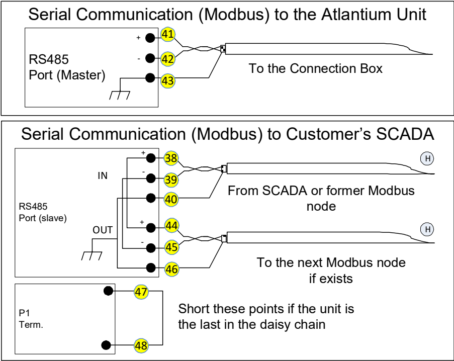
Figure 5-34: Serial Communication (Modbus) Connections
